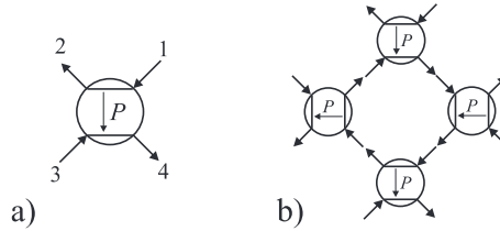
Fig. 1. a) Node of the network with two incoming and two outgoing directed channels. The channels 1 \rightarrow 2 and 3 \rightarrow 4 are treated like edge channels with backscattering, where P = R/T according to the Landauer- Büttiker formalism with R the reflection and T the transmission coefficient. b) Arrangement of the nodes for building the minimal physical element of a network, which is the closed loop of a so called magnetic bound state. The complete network is composed by putting together a sufficient number of such adjacent loops.
