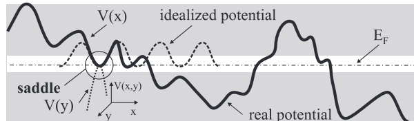
Fig. 2. Schematic one-dimensional representation ( x - profile) of a fluctuating potential together with the idealized 2D-Cosine potential with the right Taylor coefficients for representing the encircled saddle.
